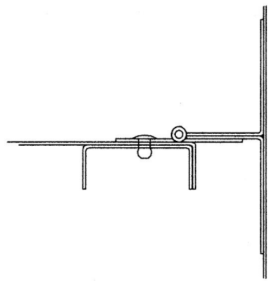
piano hinge fastener detail
