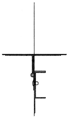
piano hinge fastener detail
